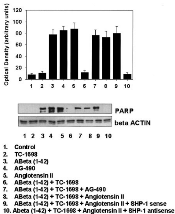
Fig. 8. Effects of SHP-1 antisense on TC-1698-induced protection against A\beta - and Ang II-induced apoptosis. PARP expression was measured from lysates of cells treated with A\beta (1-42) peptide and/or Ang II in the presence or absence of TC-1698 and/or SHP-1 antisense. Results shown for each immunoblot are representative of three immunoblots.
