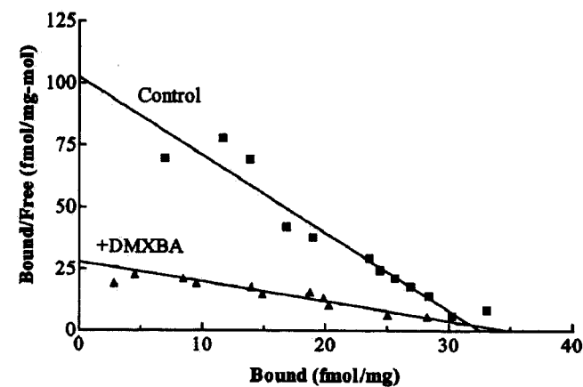
Fig. 4. DMXBA is a competitive inhibitor of specific binding of 125 I-BTX at rat brain \alpha 7 nicotinic receptors. The binding of this radiolabeled neurotoxin, measured alone and in the presence of DMXBA, is presented as a Scatchard plot. The mean K d for 125 I-BTX binding, obtained from eight saturation experiments, was 0.32 \pm 0.04 nM. Each saturation curve (data not shown) was fitted by a nonlinear least-squares method as described in the Graph-Pad Prism manual. The K i calculated for DMXBA inhibition of iodinated BTX binding in these saturation experiments was 173 nM.
