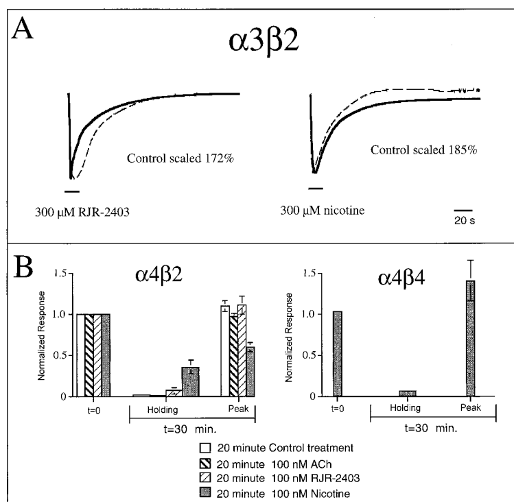
FIG. 4. A: Representative responses of \alpha 3\beta 2 -expressing oocytes to RJR-2403 and nicotine at the indicated concentrations. Responses are compared with the ACh control responses recorded immediately before the experimental drug applications. Control ACh responses have been increased in scale by the indicated factors to facilitate waveform comparisons. Bars below the traces indicate the period of agonist application. Each trace is 200 s of data. B: The effects of prolonged exposure to low agonist concentrations in \alpha 4\beta 2 - or \alpha 4\beta 4 -expressing oocytes. Control 30 \mu M ACh responses were measured at time zero and used to normalize the holding currents and subsequent ACh responses that followed 20-min applications of the drugs and 10-min wash periods. Note that only nicotine applied to \alpha 4\beta 2 receptors produced significant elevations in holding current and decreases in subsequent ACh responses. Increases in \alpha 4\beta 2 holding current induced by 100 nM nicotine ranged from 100 to 1,000 nA and were proportionate to the levels of receptor expression (i.e., control ACh responses) in the individual cells. The prolonged incubations with other agonists produced changes in holding current that were usually <100 nA and comparable with the drift in holding current when cells were held in Ringer's solution.
