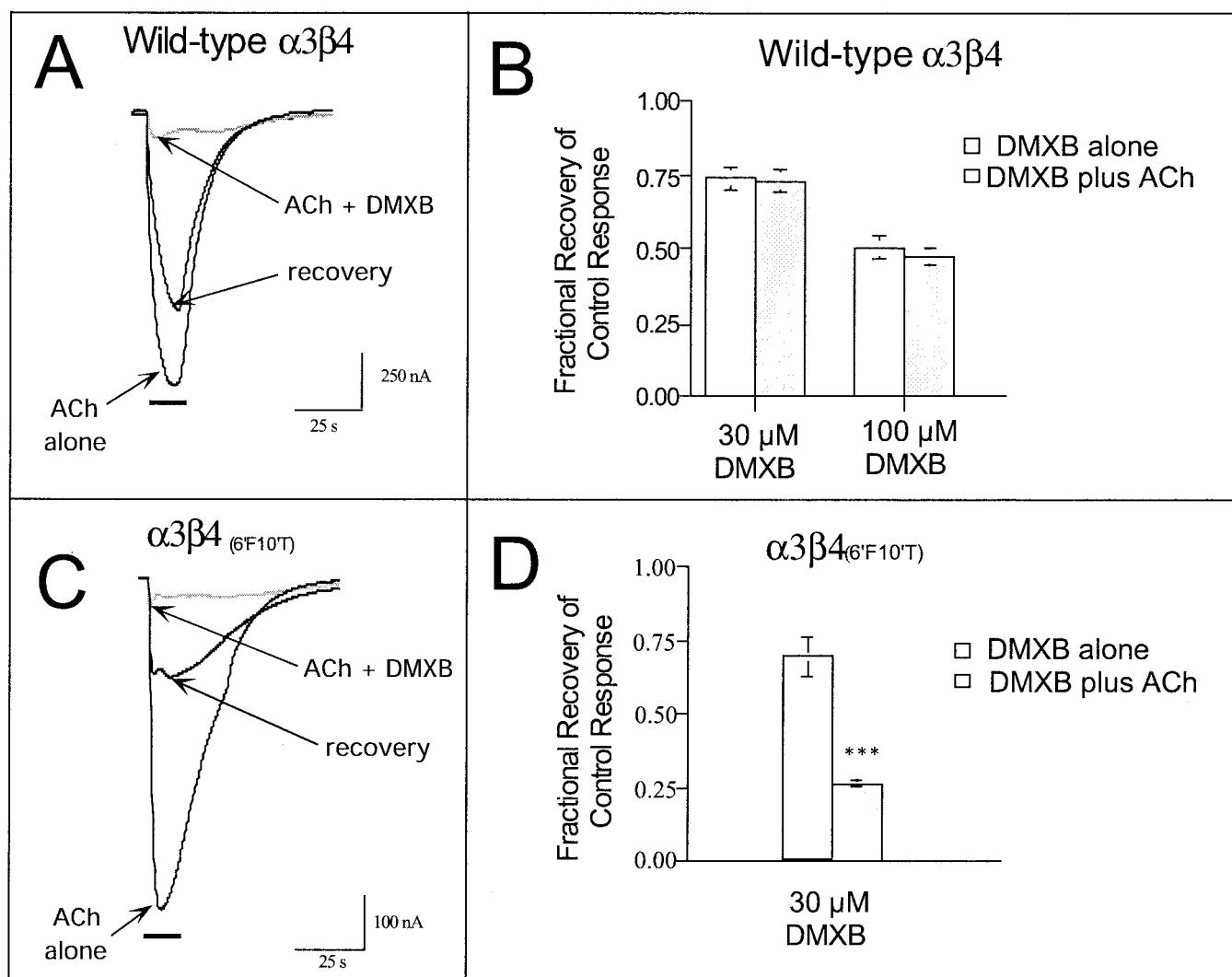
Fig. 5. Use dependence of inhibition by DMXB. A, raw data obtained from an oocyte expressing wild-type \alpha 3\beta 4 receptors. The cell was first stimulated with 100 \mu\text{M} ACh alone (left arrow) and then with 30 \mu\text{M} DMXB in combination with 100 \mu\text{M} ACh (thick gray trace). After a 5-min wash, the cell was retested with 100 \mu\text{M} ACh (recovery, right arrow). B, data obtained from oocytes expressing wild-type \alpha 3\beta 4 receptors treated with 30 or 100 \mu\text{M} DMXB alone or in combination with 100 \mu\text{M} ACh. After a 5-min wash, the cells were then reevaluated for their response to control applications of 100 \mu\text{M} ACh. The data plotted represent average residual ACh control responses of at least four oocytes. C, raw data obtained from an oocyte expressing wild-type \alpha 3\beta 4(6'F10'T) receptors. The cell was first stimulated with 100 \mu\text{M} ACh alone (left arrow) and then with 30 \mu\text{M} DMXB in combination with 100 \mu\text{M} ACh (thick gray trace). After a 5-min wash, the cell was retested with 100 \mu\text{M} ACh (recovery, right arrow). D, data obtained from oocytes expressing \alpha 3\beta 4(6'F10'T) receptors treated with 30 \mu\text{M} DMXB alone or in combination with 100 \mu\text{M} ACh. After a 5-min wash, the cells were then reevaluated for their response to control applications of 100 \mu\text{M} ACh. The data plotted represent average residual ACh control responses of at least four oocytes.
