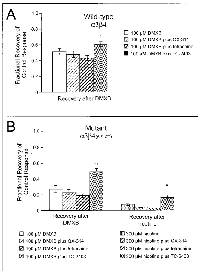
Fig. 6. Protection of receptor function. A, oocytes expressing wild-type \alpha 3\beta 4 receptors were treated with 100 \mu M DMXB alone or in the presence of 20 \mu M QX-314, 100 \mu M tetracaine, or TC-2403. Control 100 \mu M ACh responses were then measured after a 5-min wash and compared with the initial ACh control responses. Only the coapplication of 100 \mu M TC-2403 was effective at decreasing the residual inhibition measured after the application of 100 \mu M DMXB. B, the bars on the right illustrate the results obtained when oocytes expressing \alpha 3\beta 4(6'F10'T) receptors were treated with 100 \mu M DMXB alone or in coapplication with 200 \mu M QX-314, 100 \mu M tetracaine, or 100 \mu M TC-2403. Control 100 \mu M ACh responses were measured after a 5-min wash and compared with the initial ACh control responses. Only the coapplication of 100 \mu M TC-2403 was effective at decreasing the residual inhibition measured after the application of 100 \mu M DMXB. The bars on the left illustrate the results obtained when oocytes expressing \alpha 3\beta 4(6'F10'T) receptors were treated with 300 \mu M nicotine alone or in coapplication with 200 \mu M QX-314, 300 \mu M tetracaine, or 100 \mu M TC-2403. Note that nicotine is an efficacious agonist for the mutant receptor, and we have shown that the inhibitory effects of tetracaine on the mutant receptor are decreased with high levels of agonist activation (Papke et al., 2001). Therefore, we chose to use a somewhat higher concentration of tetracaine in this nicotine protection experiment. Control 100 \mu M ACh responses were measured after a 5-min wash and compared with the initial ACh control responses. Only the coapplication of 100 \mu M TC-2403 was effective at decreasing the residual inhibition measured after the application of 300 \mu M nicotine. Note that for both panels A and B, cells were pre-equilibrated for 12 s with QX-314, tetracaine, or TC-2403 before coapplication of DMXB or nicotine with the indicated agents.
