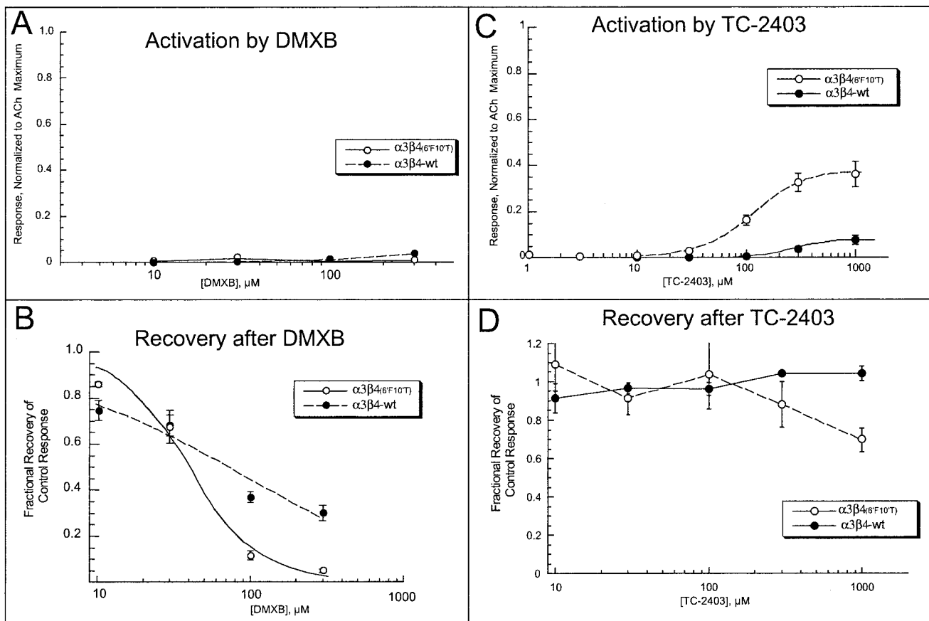
Fig. 3. Concentration-response curves for the effect of DMXB and TC-2403 on \alpha 3\beta 4 and \alpha 3\beta 4(6'F10'T) receptors. A, the concentration-response relationship for the activation of the peak currents by DMXB. Data are expressed relative to ACh maximum responses (see Materials and Methods ). B, the concentration-response relationship for the recovery of control ACh response amplitude measured 5 min after DMXB was applied at the indicated concentrations. C, the concentration-response relationship for the activation of the peak currents by TC-2403. Data are expressed relative to ACh maximum responses (see Materials and Methods ). D, the concentration-response relationship for the recovery of control ACh response amplitude measured 5 min after TC-2403 was applied at the indicated concentrations. Each point represents the average normalized response of at least four cells.
