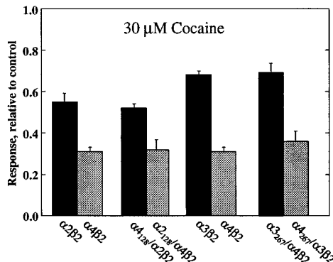
Fig. 6. Cocaine inhibition of \alpha subunit chimeras. A , sequence alignment of nAChR \alpha subunits. Identical amino acids are shaded black. Conservative differences are in gray. The three principle loops believed to participate in agonist binding and the four putative transmembrane domains are denoted. The conserved restriction sites for PstI and BstXI used in constructing the \alpha 2/4 and \alpha 3/4 subunit chimeras are also shown. Numbering is relative to the vicinal cysteines (192 and 193) indicated by the asterisk. B , schematic depicting structure of \alpha subunit chimeras. Chimeric subunits were created using homologous restriction sites shared between either \alpha 2 and \alpha 4 (PstI) or \alpha 3 and \alpha 4 (BstXI). C , responses of \alpha subunit chimeric receptors to 30 \mu\text{M} ACh in the absence and presence (middle trace) of 30 \mu\text{M} cocaine. The bar above the first trace shows the timing of the agonist application. D , the mean response of nAChR subtypes to the coapplication of ACh with cocaine. Each column represents the mean relative response ( \pm S.E.) of four or more oocytes to the application of 30 \mu\text{M} ACh with 30 \mu\text{M} cocaine.
