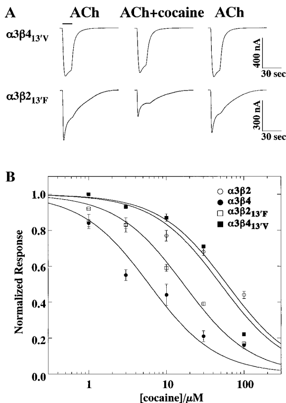
Fig. 3. Cocaine inhibition of 13' \beta subunit mutant nAChRs. A, responses of 13' mutant receptors to 30 \mu M ACh in the absence and presence (middle trace) of 10 \mu M cocaine. Each application is separated by approximately 4 min and the bar above the first trace shows the timing of the agonist application. B, concentration dependence of cocaine inhibition of nAChR. Each data point represents the mean response ( \pm S.E.) of at least four oocytes to the coapplication of 30 \mu M ACh with varying concentrations of cocaine and is normalized to a 30 \mu M ACh control response.
