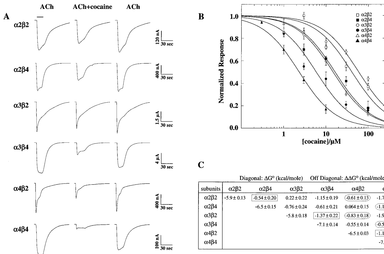
Fig. 1. Cocaine inhibition of nAChR subtypes. A, responses of neuronal nAChRs to 30 \mu M ACh in the absence and presence (middle trace) of 10 \mu M cocaine. ACh was applied for 15 s in each case, and the bar above the first trace (upper left) shows the timing of the application. In this figure and subsequent figures, the trace at left is the response to a control application of ACh alone, the middle trace is the response to application of ACh with cocaine, and the trace at right is the response to a second control application of ACh representing recovery from inhibition. Each application is separated by approximately 4 min. B, concentration dependence of cocaine inhibition of nAChR. Each data point represents the mean response of at least four oocytes to the coapplication of 30 \mu M ACh with varying concentrations of cocaine relative to 30 \mu M ACh alone. C, \Delta G^\circ and \Delta\Delta G^\circ values associated with cocaine binding to nAChR subunit combinations. Boxed values indicate \Delta\Delta G^\circ values for comparisons of \beta 2 - versus \beta 4 -containing receptors, and circles indicate \Delta\Delta G^\circ values for \alpha 4 - versus \alpha 3 - and \alpha 2 -containing receptors.
