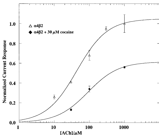
Fig. 5. Cocaine inhibition of \alpha 4\beta 2 receptors as a function of agonist concentration. Acetylcholine (10 \mu M–1 mM) was applied in the absence and presence of 30 \mu M cocaine. Each data point is expressed relative to the ACh maximum and represents the mean ( \pm S.E.) of three to six responses.
