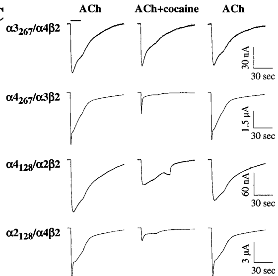
Fig. 6. Cocaine inhibition of \alpha subunit chimeras. A , sequence alignment of nAChR \alpha subunits. Identical amino acids are shaded black. Conservative differences are in gray. The three principle loops believed to participate in agonist binding and the four putative transmembrane domains are denoted. The conserved restriction sites for PstI and BstXI used in constructing the \alpha 2/4 and \alpha 3/4 subunit chimeras are also shown. Numbering is relative to the vicinal cysteines (192 and 193) indicated by the asterisk. B , schematic depicting structure of \alpha subunit chimeras. Chimeric subunits were created using homologous restriction sites shared between either \alpha 2 and \alpha 4 (PstI) or \alpha 3 and \alpha 4 (BstXI). C , responses of \alpha subunit chimeric receptors to 30 \mu\text{M} ACh in the absence and presence (middle trace) of 30 \mu\text{M} cocaine. The bar above the first trace shows the timing of the agonist application. D , the mean response of nAChR subtypes to the coapplication of ACh with cocaine. Each column represents the mean relative response ( \pm S.E.) of four or more oocytes to the application of 30 \mu\text{M} ACh with 30 \mu\text{M} cocaine.
