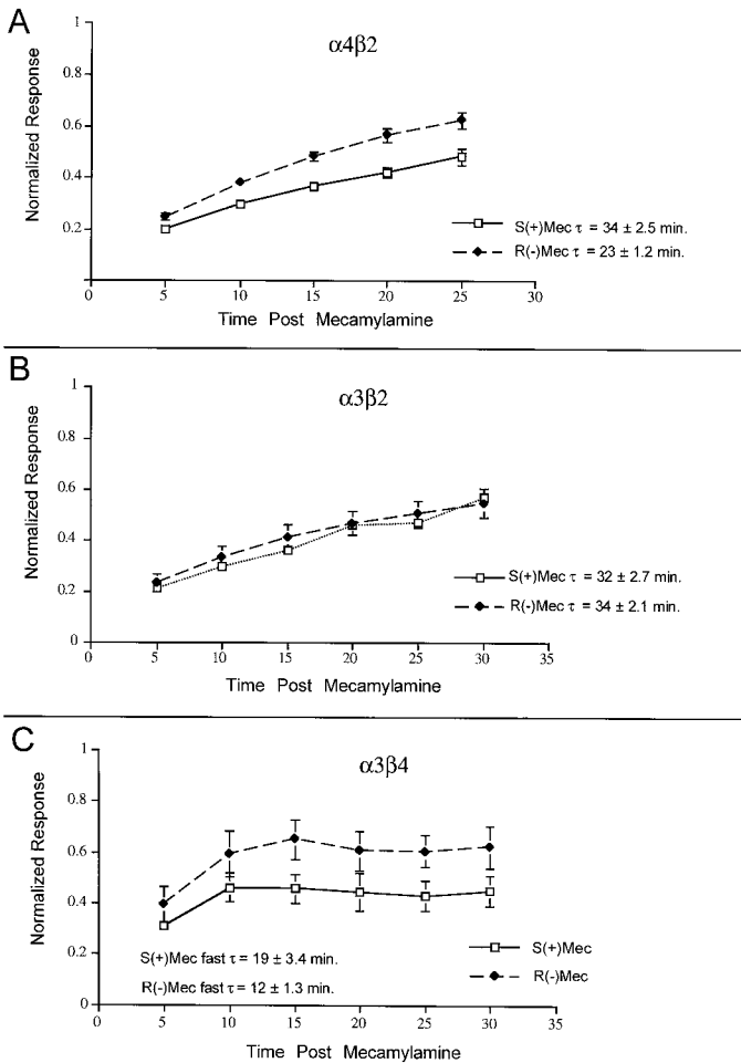
Fig. 6. The recovery of ACh control responses. Cells were monitored for their responses to control applications of ACh at 5-min intervals after 10 \mu M mecamylamine (Mec) was coapplied with ACh on: A, \alpha 4 \beta 2 receptors; B, \alpha 3 \beta 2 receptors; and C, \alpha 3 \beta 4 receptors. Data from each oocyte were normalized to that cell's response to ACh alone. Each point represents the average normalized response of at least four cells.
