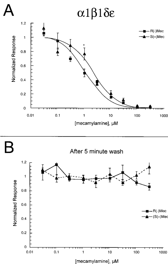
Fig. 4. Effect of mecamylamine (Mec) on ACh-evoked currents in oocytes expressing the \alpha 1\beta 1\delta\epsilon subunits of the adult muscle-type nAChR. A , concentration-response relationship for mecamylamine's inhibition of the peak currents of muscle-type receptors when 30 \mu\text{M} ACh was coapplied with mecamylamine at the indicated concentrations. Data from each oocyte were normalized to that cell's response to 3 \mu\text{M} ACh alone. All cells were pre-equilibrated with mecamylamine at the indicated concentration for 10 s before the coapplication of agonist with antagonist. Each point represents the average normalized response of at least four cells. B , amplitude of 3 \mu\text{M} ACh control responses obtained 5 min after the application of ACh and mecamylamine at the indicated concentrations. In contrast to the residual inhibition seen with neuronal nAChR receptors, the inhibition of muscle-type receptors was essentially fully reversible.
