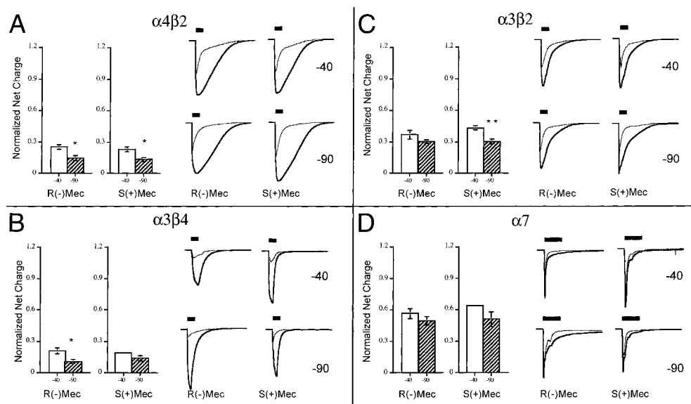
Fig. 9. Voltage dependence of mecamylamine (Mec)-induced inhibition of net charge during the coapplication of ACh and either S(+) -mecamylamine or R(-) -mecamylamine. Mecamylamine was coapplied with agonist at either -40 or -90 mV. Inhibition of net charge was calculated relative to the net charge in the initial control ACh responses. Representative traces are shown to the right of the bar graphs. Drug applications were 12 s in duration and correspond to the bars. Note that the rapidly desensitizing \alpha 7 receptor-mediated responses are shown at an expanded time scale. In all cases, the response obtained in the presence of mecamylamine is shown as the thin line contained within the thick line that corresponds to the control ACh response obtained 5 min before the ACh/mecamylamine coapplication. The concentrations of mecamylamine used were: A, 5 \mu M for \alpha 4\beta 2 receptors; B, 1 \mu M for \alpha 3\beta 4 receptors; C, 5 \mu M for \alpha 3\beta 2 receptors; and D, 10 \mu M for \alpha 7 receptors. Each point represents measurements from at least four cells. Analysis was conducted on the same responses that were represented in Fig. 8 in terms of peak amplitude. However, more significant effects of voltage were revealed when the data were analyzed in terms of net charge rather than peak currents. Columns marked with a double asterisk were determined to be significantly different from the corresponding -40 mV control data at p < 0.01 by unpaired t tests.
