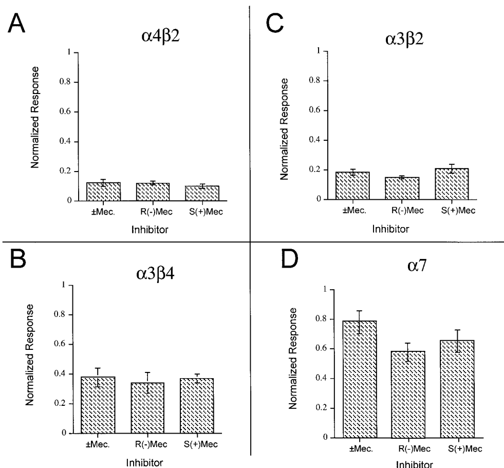
Fig. 2. Residual effects of mecamlamine (Mec) on ACh control responses. Control ACh responses 5 min after the coapplication of 10 \mu M mecamlamine to \alpha 4\beta 2 receptors (A), \alpha 3\beta 4 receptors (B), \alpha 3\beta 2 receptors (C), and \alpha 7 receptors (D). Control ACh concentrations used for these receptor subtypes were 30 \mu M, 100 \mu M, 30 \mu M, and 300 \mu M, respectively. Each bar represents the average normalized responses of four to seven cells.
