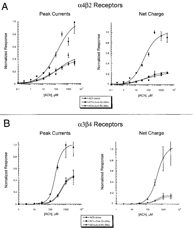
Fig. 7. Competition studies. A, ACh concentration response curves for \alpha 4 \beta 2 receptors were determined with ACh alone or ACh coapplied with 3 \mu M S(+) -mecamylamine or R(-) -mecamylamine. Data were initially normalized to the 30 \mu M ACh responses obtained in the same cells and then scaled by the ratio of 30 \mu M ACh control responses to the maximal ACh responses, obtained with 3 mM ACh. Each point represents the average normalized response of at least four cells. Data in the left plot show the effect of mecamylamine (Mec) on peak currents. Data in the right plot show the effect of mecamylamine on the net charge during a coapplication of ACh and mecamylamine, normalized to the net charge in the responses to ACh alone. B, ACh concentration-response curves for \alpha 3 \beta 4 receptors were determined with ACh alone or ACh coapplied with 3 \mu M S(+) -mecamylamine or R(-) -mecamylamine. Data were initially normalized to the 100 \mu M ACh responses obtained in the same cells and then scaled by the ratio of the 100 \mu M ACh control responses to the maximal ACh responses, obtained with 3 mM ACh. Each point represents the average normalized response of at least four cells. Data in the left plot show the effect of mecamylamine on peak currents. Data in the right plot show the effect of mecamylamine on the net charge during a coapplication of ACh and mecamylamine, normalized to the net charge in the responses to ACh alone.
